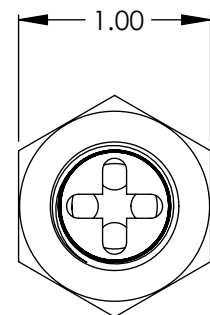
2300 Series - 3MP
